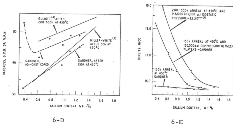
Fig 6-D Effect of Gallium Content on Hardness
